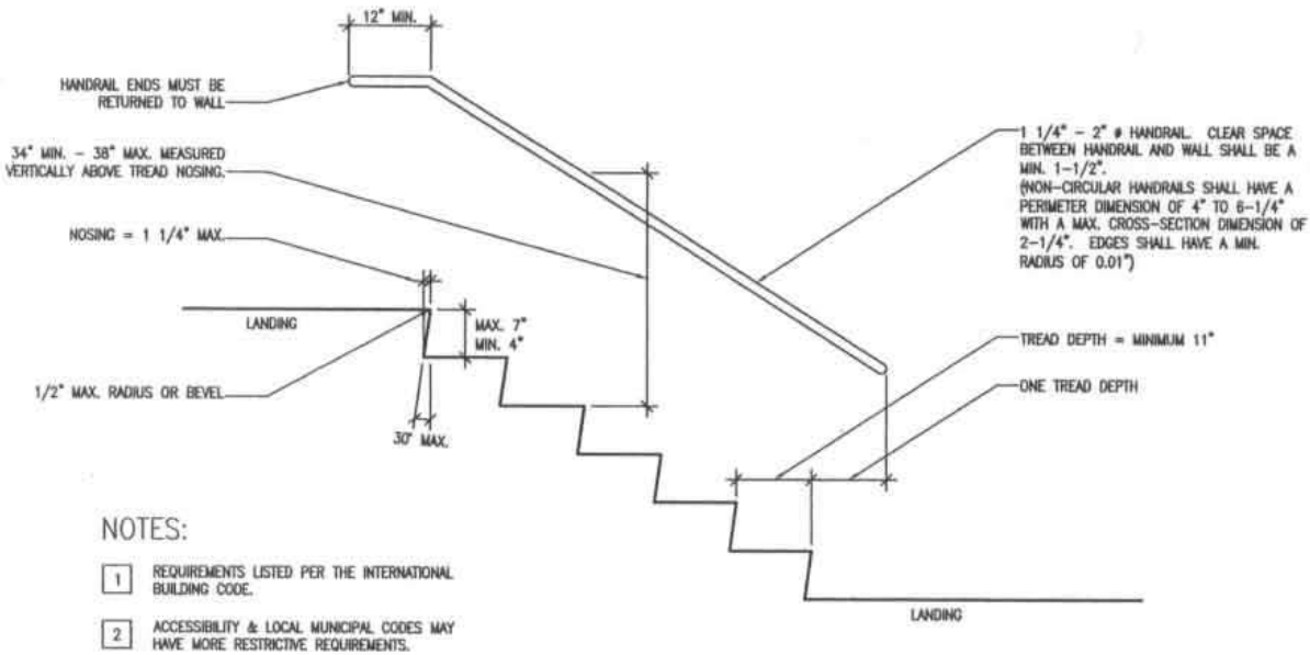
1 STAIR SECTION NTS
